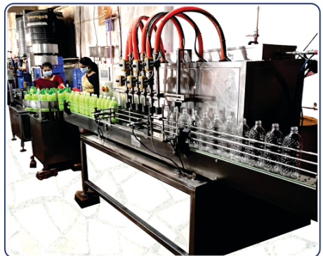
FLOOR CLEANER AUTOMATIC FILLING MACHINE
